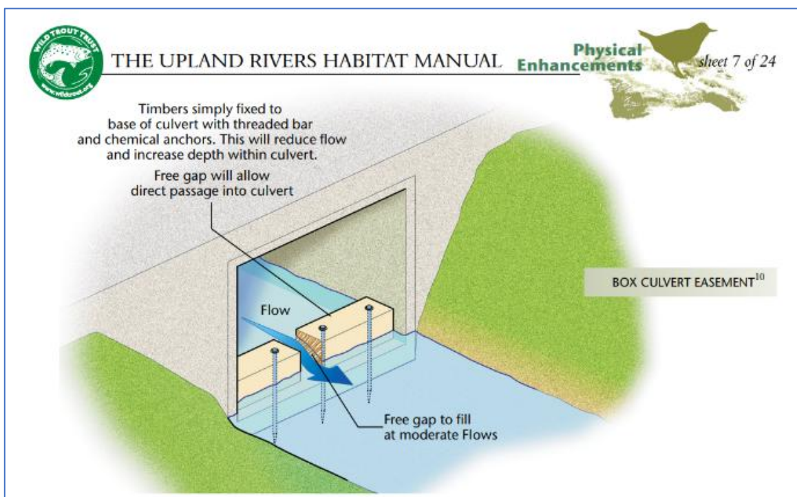
Figure 4 An example of a simple intervention to raise low flow levels in a culvert for fish passage. The bed gradient in the culvert will dictate how long a culvert this would work for. This could be replicated downstream of the low weir created in picture 9, to 'drown' it out by elevating water levels just downstream.
